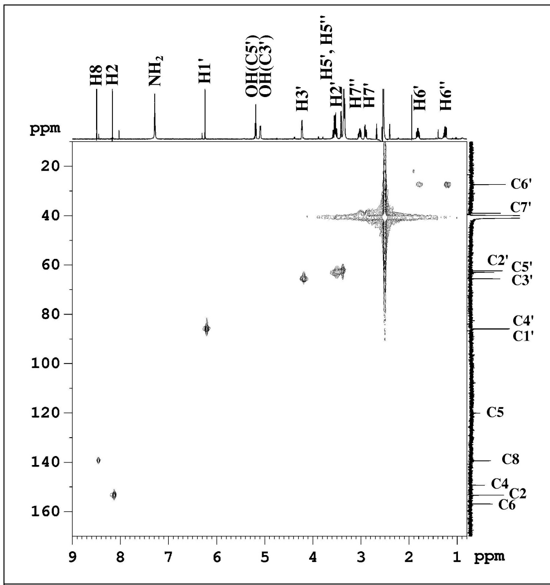
Figure S2. HMQC spectrum of compound 14a.
